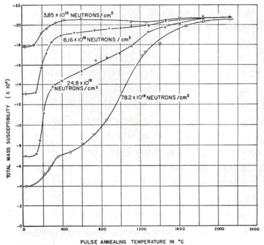
FIG. 13. Pulse-annealing spectrum of the susceptibility.
