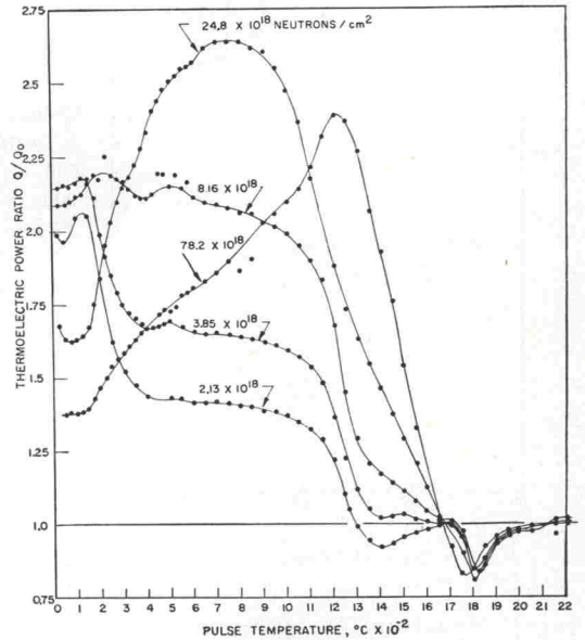
FIG. 12. Pulse-annealing spectrum of the thermoelectric power.
