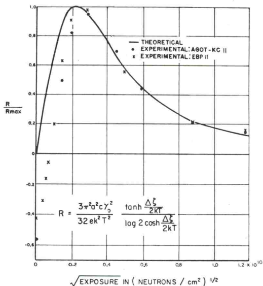
FIG. 1. The Hall coefficient vs neutron exposure at room temperature.
